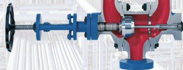
Change-over Valve
