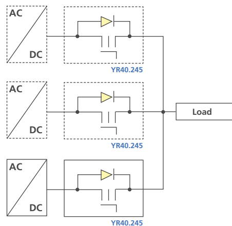
N+1-Redundancy
