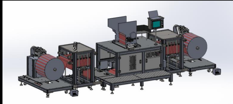
<VINYL PRINTER MACHINE>
