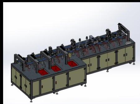
<SENSOR ASSY MACHINE 3>
