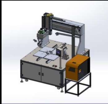
<HOTMELT DISPENSER MACHINE>
