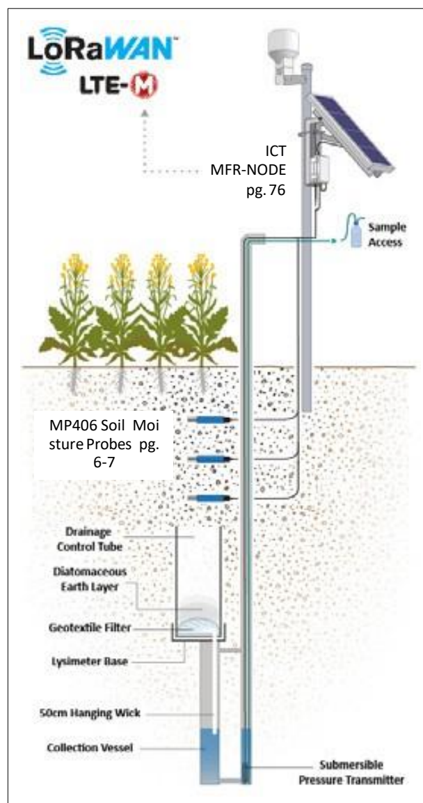
GroundTruth Lysimeter With Autosampler
