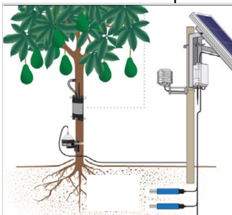
Sensor-Node Integrated Package (SNIp) for Avocado Irrigation Monitoring
