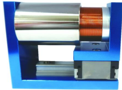
<VOICE COIL MOTOR STAGE : SFSV-L54-S10-F20>
