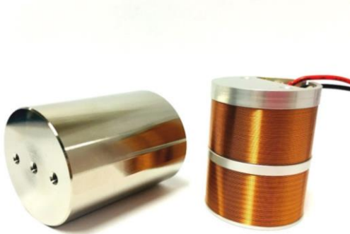
<VOICE COIL MOTOR : SFMV-L54-S10-F20>
